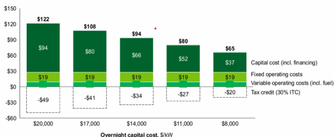
Figure 1: Impact of overnight capital costs on nuclear energy levelized cost of electricity. Source: DOE Updated Advanced Nuclear Liftoff Report
